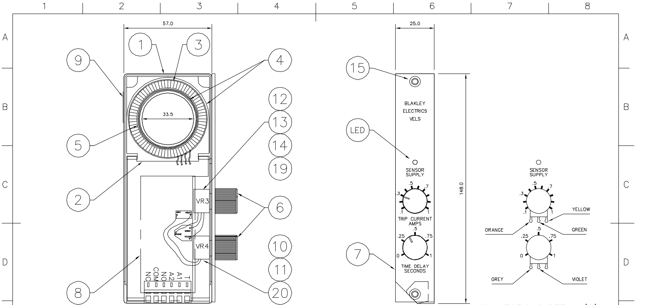
CONNECTIONS DETAIL 'A'
