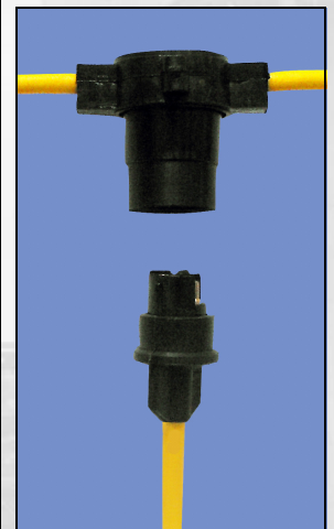
Flori-2X Adaptor Outlets are finger proof but should be capped-off if not
