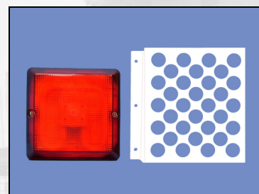
(a) Low Energy Bulkhead, 110V 16W 2D Lamp, Polycarbonate Body and Cover; (b) Metal Guard
