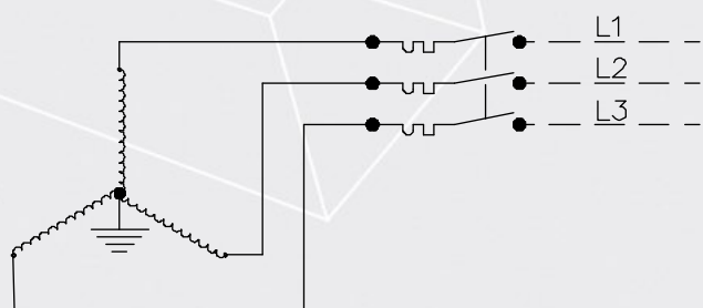
Three Phase 110V NE Supply
