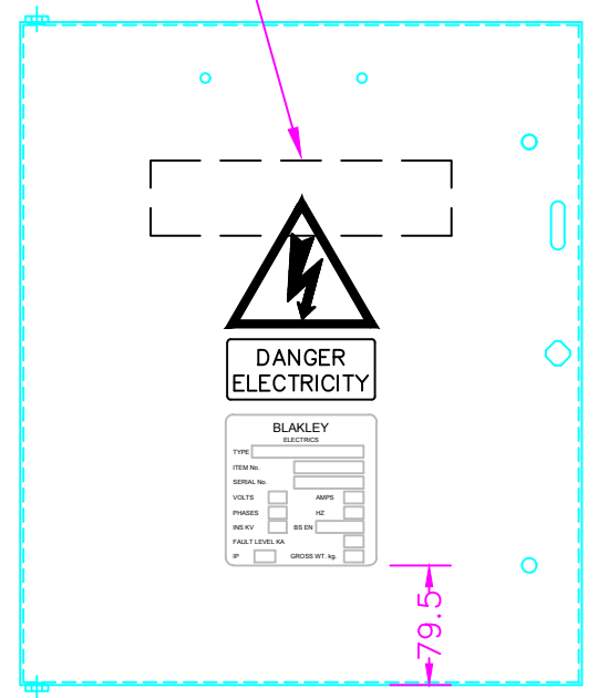
VIEW SHOWING RATING PLATE & LABEL POSITIONS ON THE DOOR
