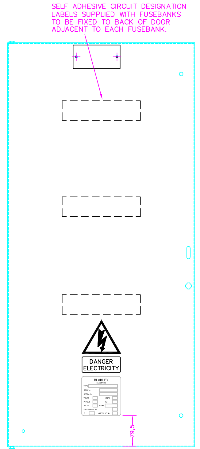
VIEW SHOWING RATING PLATE & LABEL POSITIONS ON THE DOOR BASED ON DWG: A7291400
