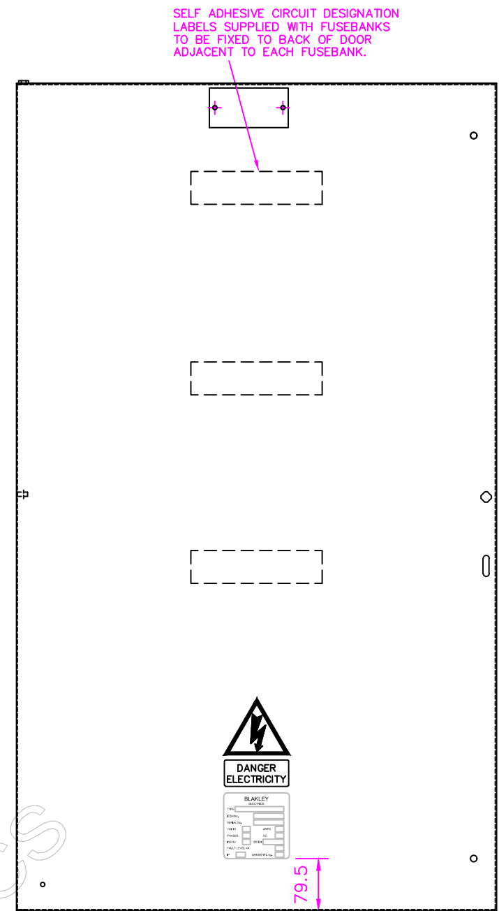
VIEW SHOWING RATING PLATE & LABEL POSITIONS ON THE DOOR
