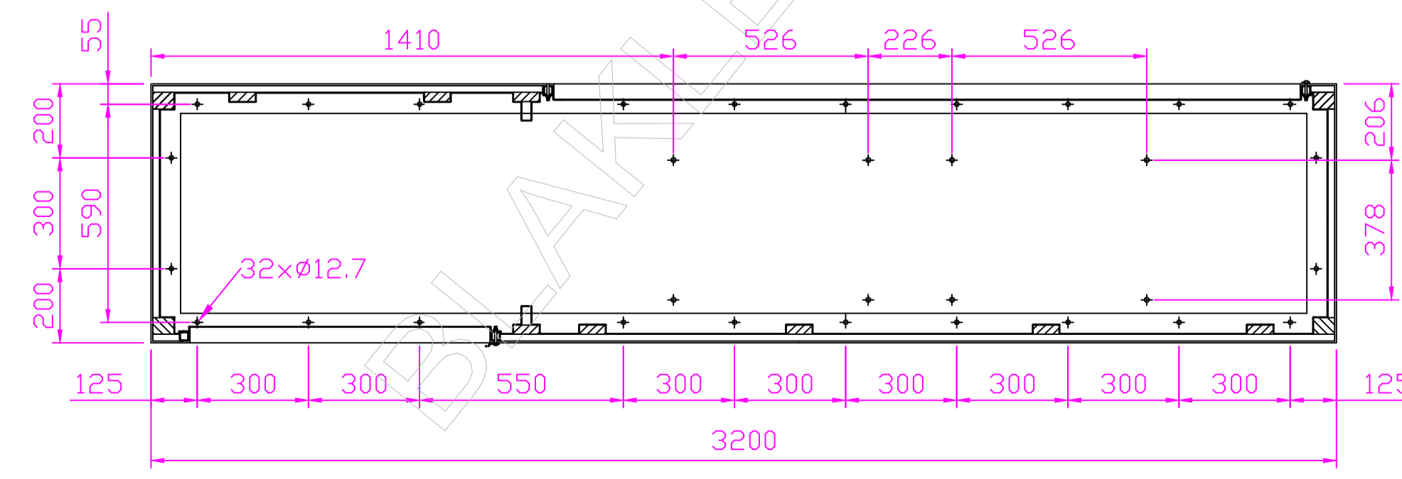
VIEW IN DIRECTION OF ARROW A FIXING DOWN DETAILS
