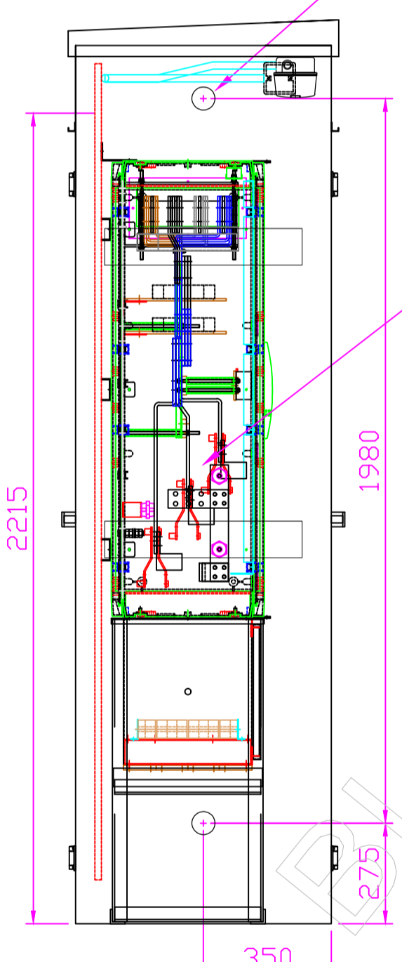
CT CHAMBER COMPARTMENT
