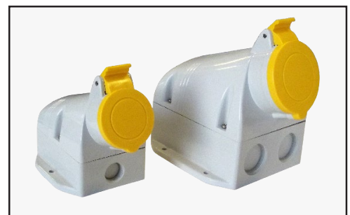
16A and 32A, 110V, 2P+E, IP44, Surface Sockets
