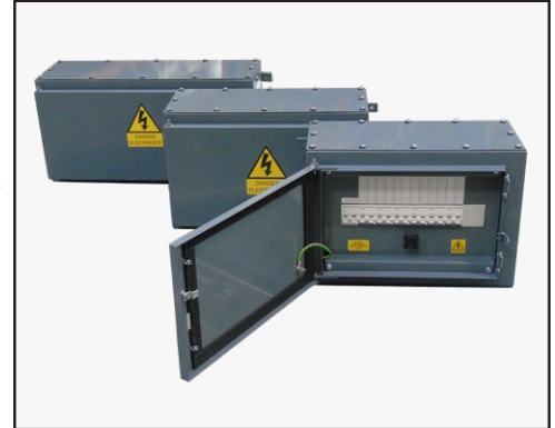
MCB Boards fitted with 6, 8 or 10 no. 16A DP Type "C" MCBs or RCBOs
